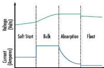
CHARGING CURVE
